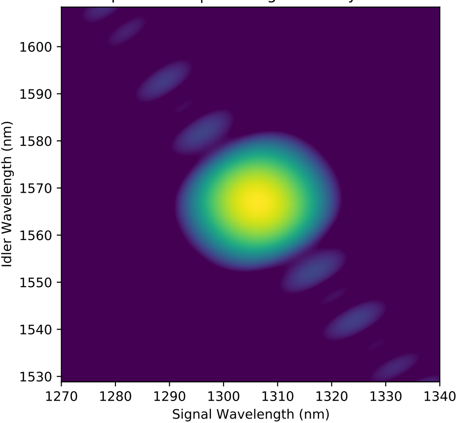
3. Optimized JSA (Theory, Log) Pump=4.40nm | Indistinguishability=0.9963
