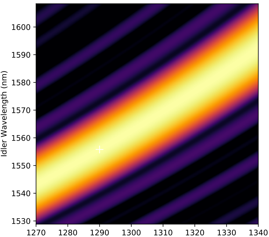
3. Optimized JSA (Theory, Log) Pump=4.40nm | Indistinguishability=0.9963
