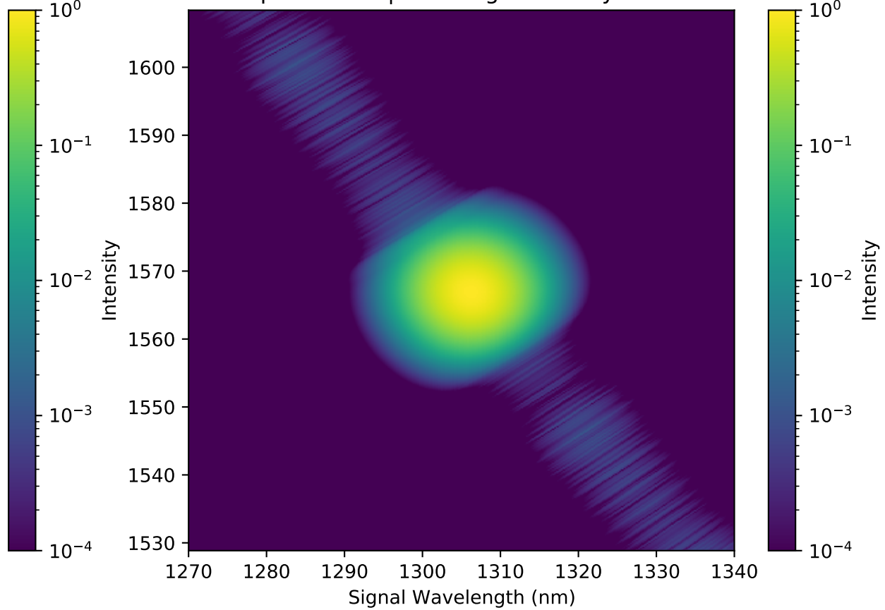
4. Optimized JSA (Exp Reconstruction, Log) Pump=4.40nm | Indistinguishability=0.9925
