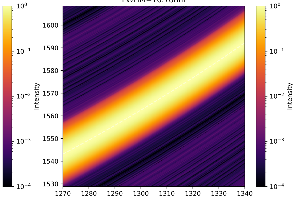
4. Optimized JSA (Exp Reconstruction, Log) Pump=4.40nm | Indistinguishability=0.9925
